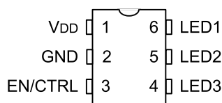
AS6503 SOT-26
